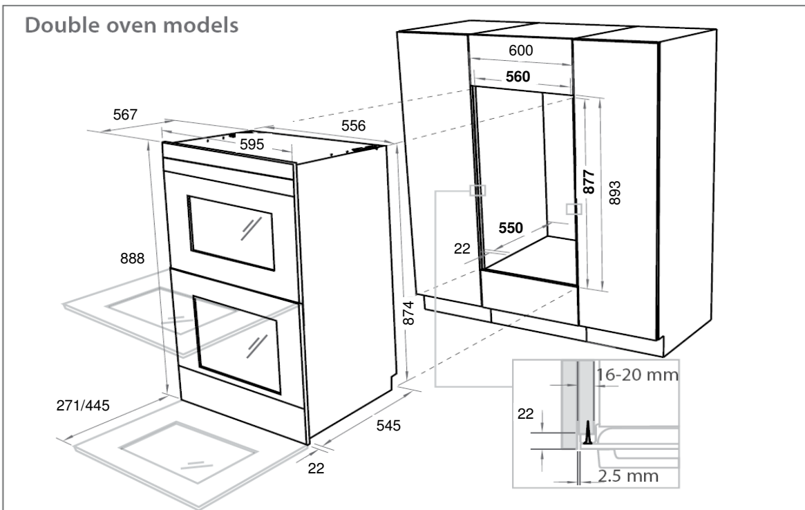
Figure 3 Double product and cabinetry dimensions
