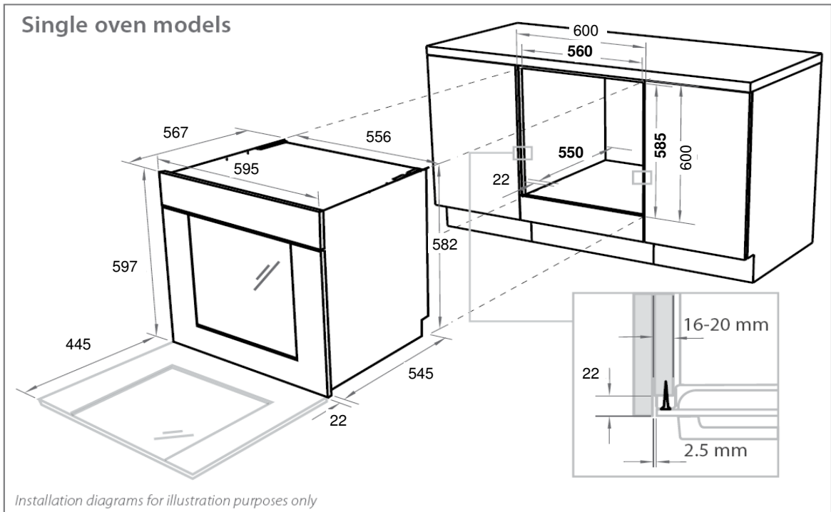
Figure 2 Single product and cabinetry dimensions
